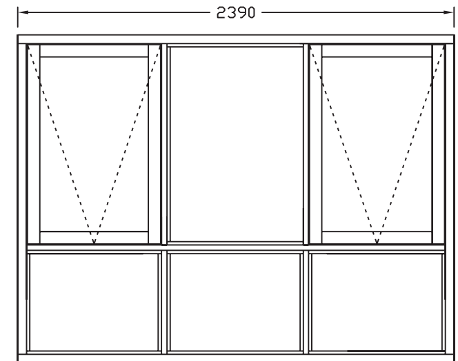
FTW 1800 X 2390 A
