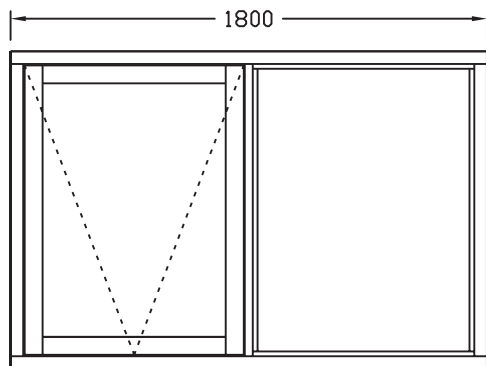
FTW 1200 X 1800 A
