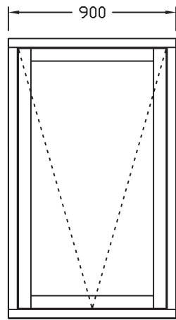
FTW 1500 X 900 A
