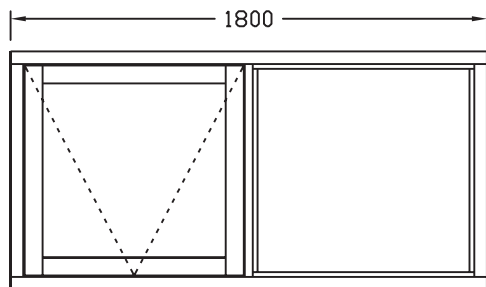
FTW 900 X 1800 A
