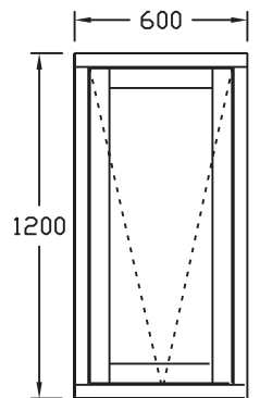
FTW 1200 X 600 A
