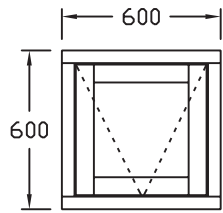
FTW 600 X 600 A
