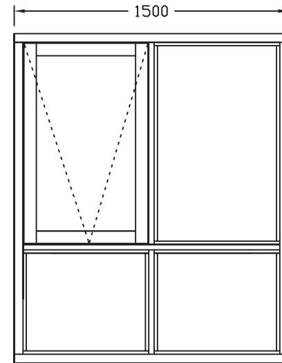
FTW 1800 X 1500 A
