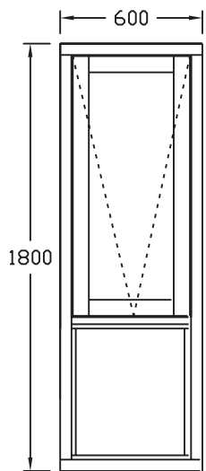
FTW 1800 X 600 A
