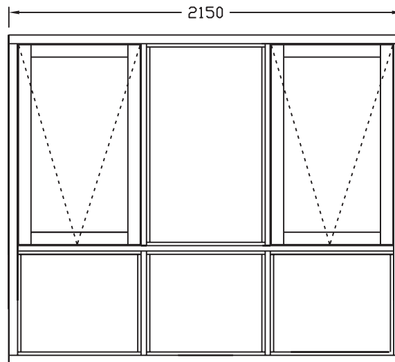
FTW 1800 X 2150 A
