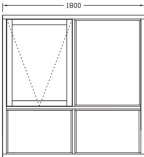
FTW 1800 X 1800 A
