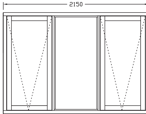
FTW 1500 X 2150 A
