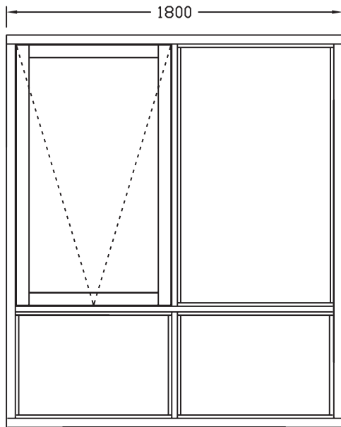
FTW 2100 X 1800 A
