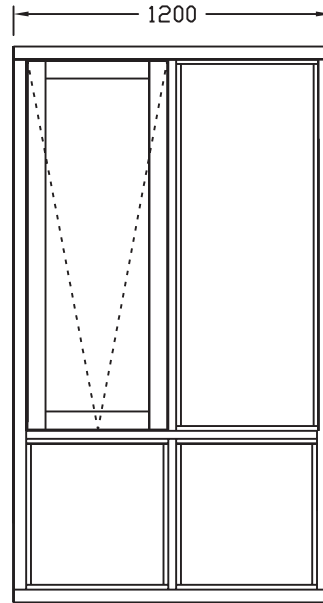
FTW 2100 X 1200 A
