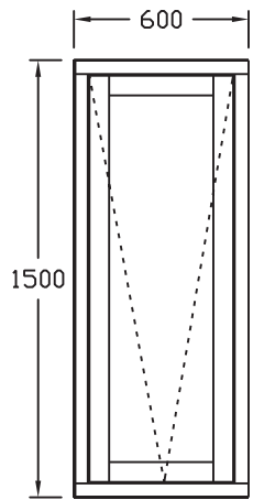
FTW 1500 X 600 A
