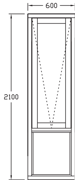
FTW 2100 X 600 A
