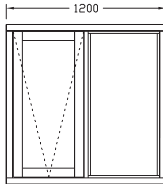
FTW 1200 X 1200 A
