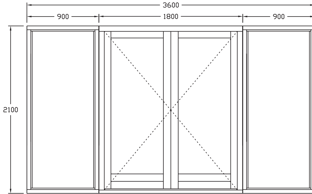
FTW 2100 X 3600 French door / Fixed Glass Combination frame
